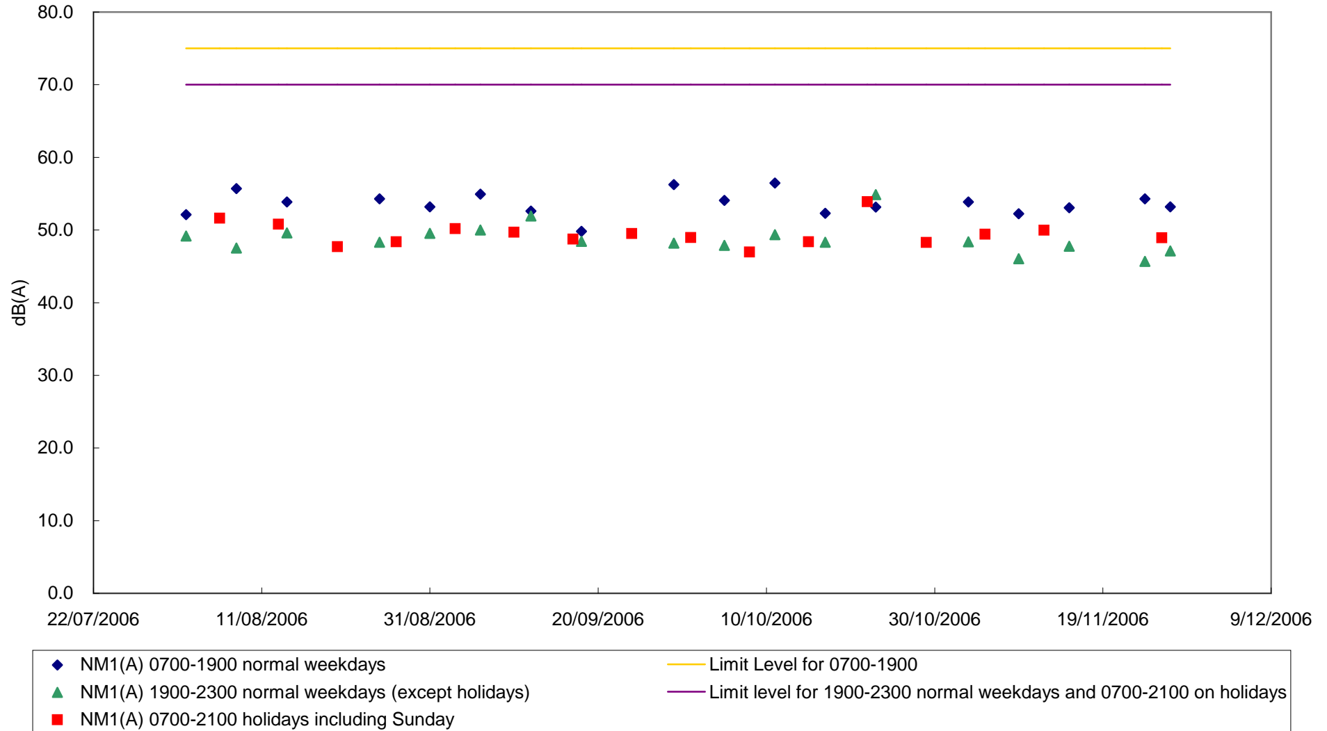
Figure 5.2 - Graphical Plot of Noise Levels at NM1(A)
